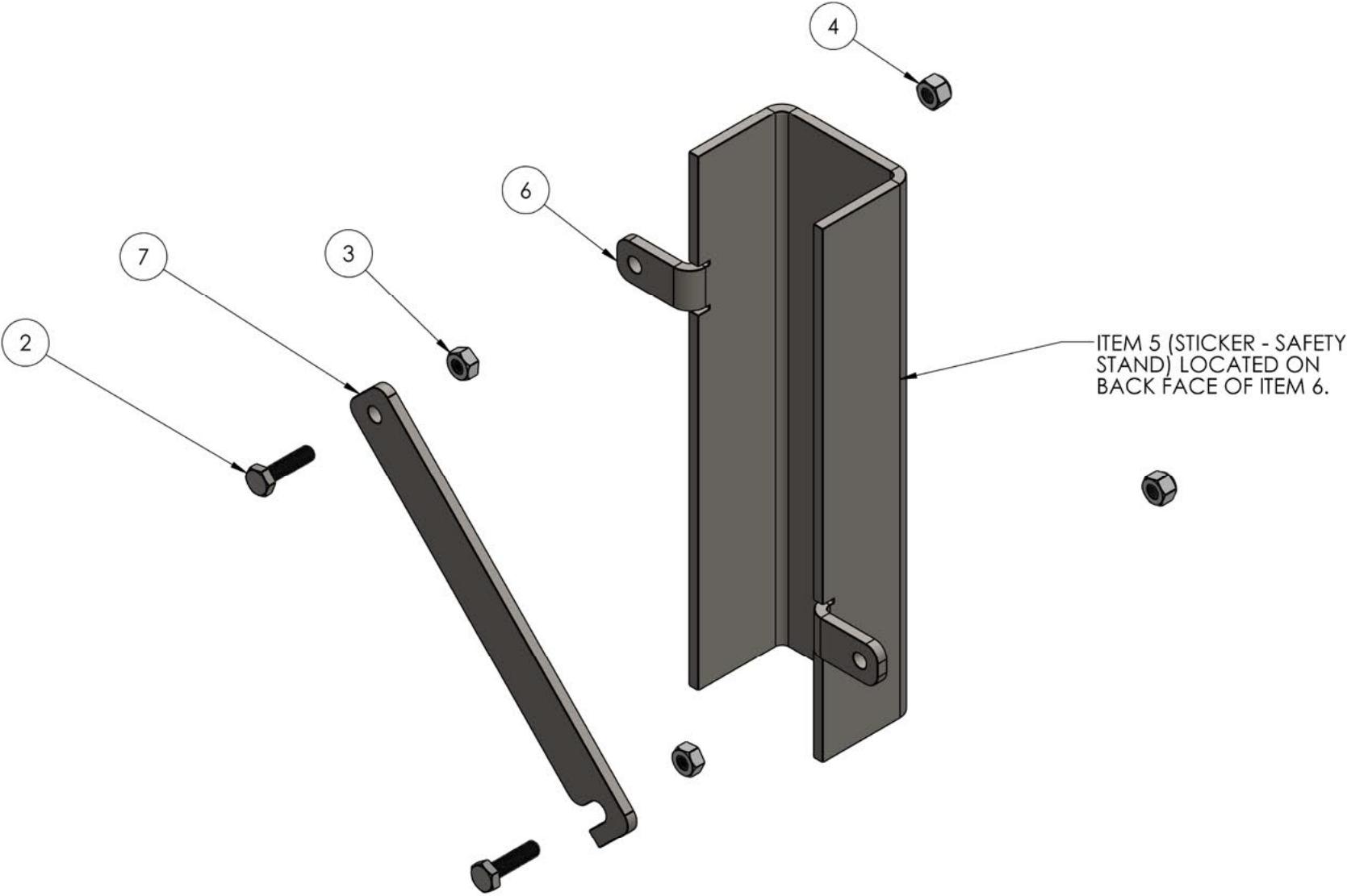
Safety Stand - Diagram 1
