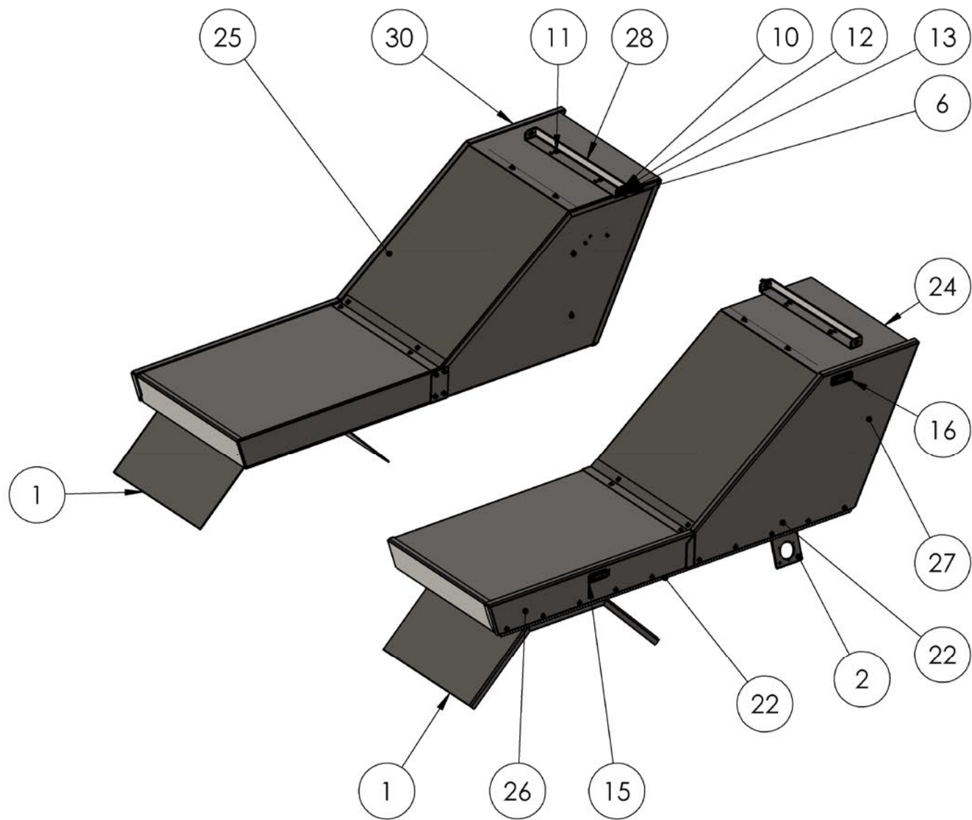
Top View - Toolboxes - Diagram 1
