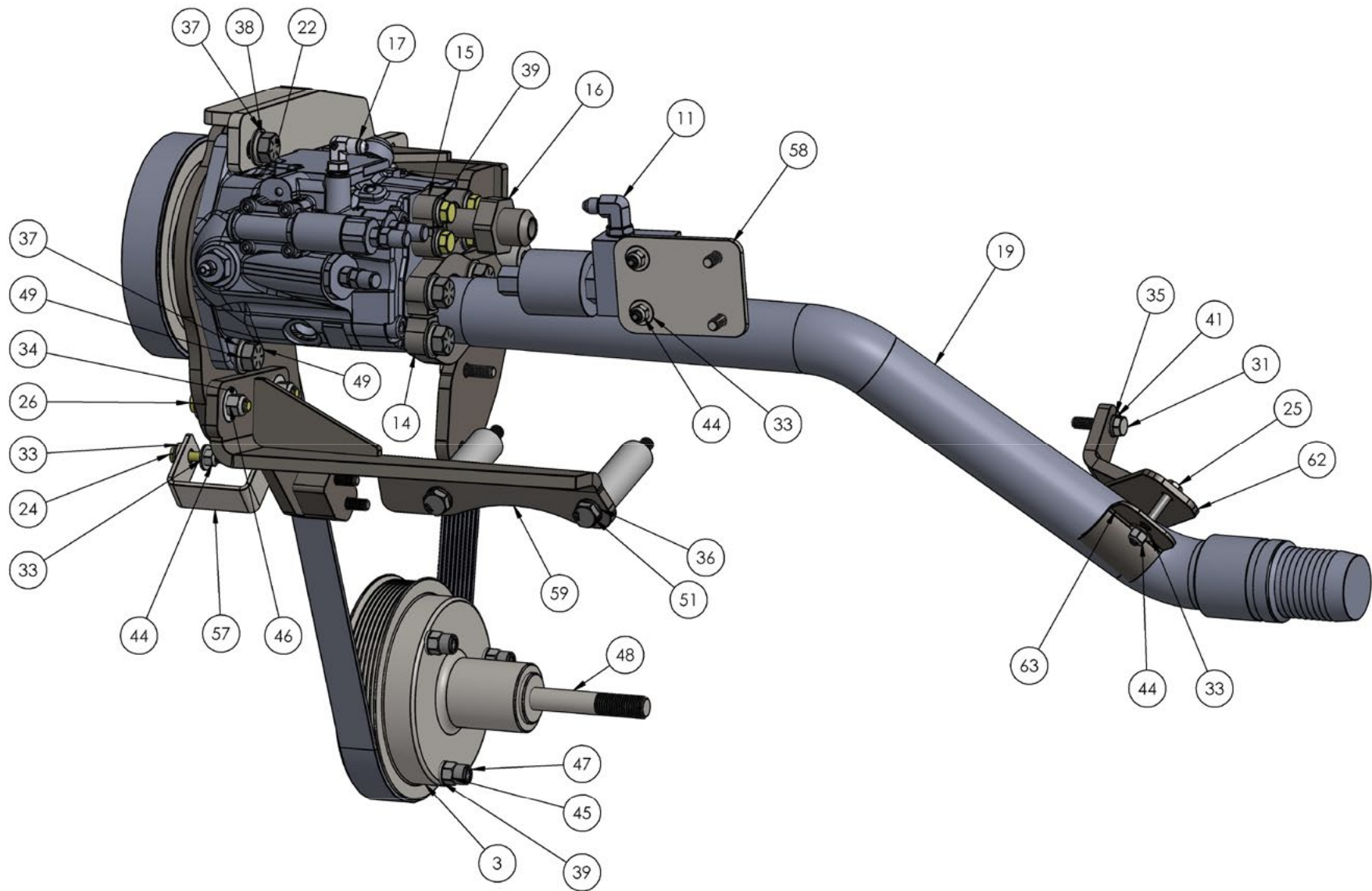
Driver Side View 2 - Pump & Belt Assembly - Diagram 2
