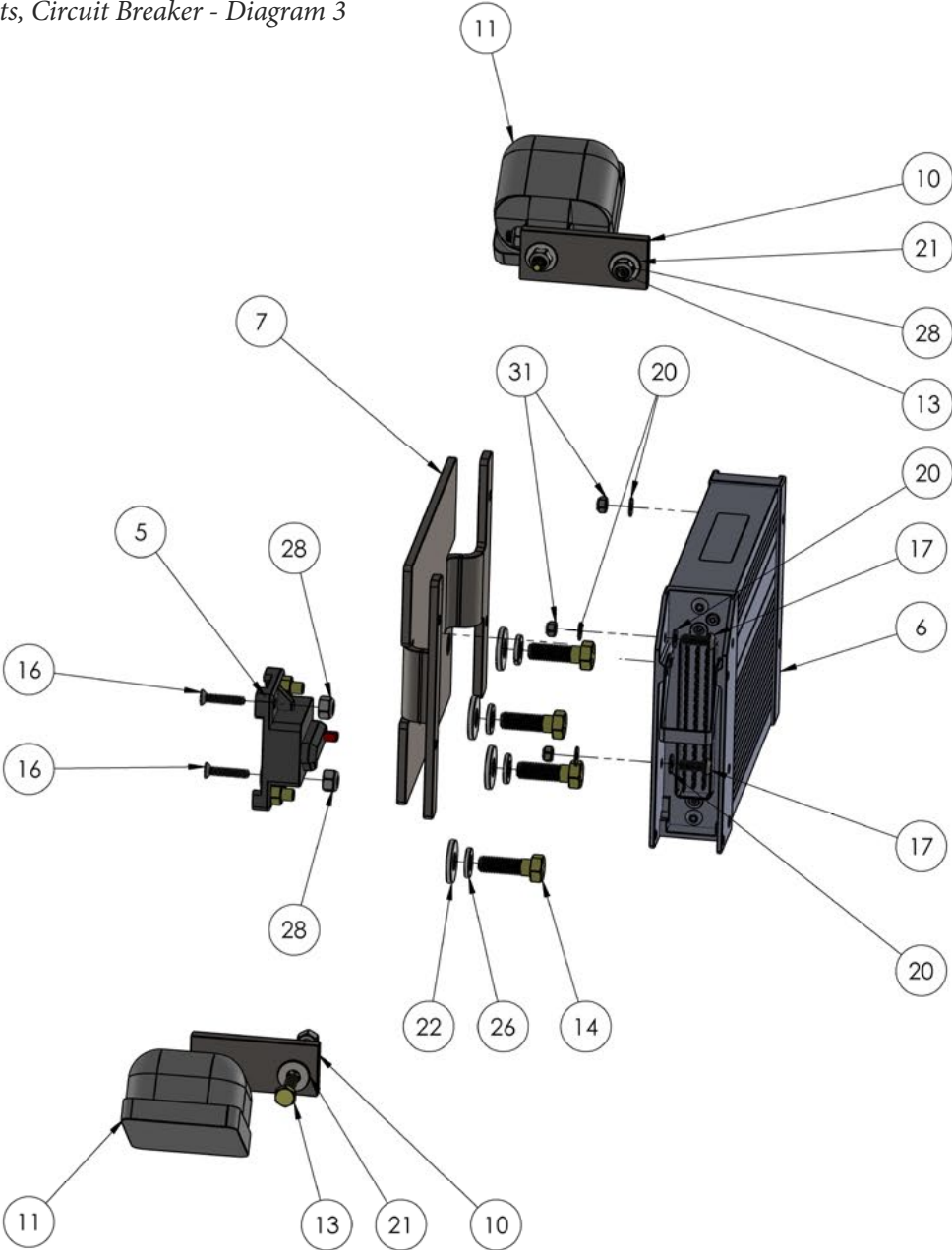
Exploded View - IFM Controller, Side Spotlights, Circuit Breaker - Diagram 3
