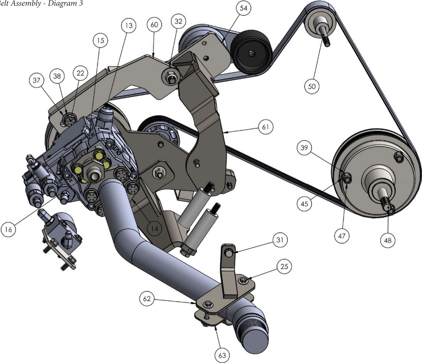
Rear View - Pump & Belt Assembly - Diagram 3
