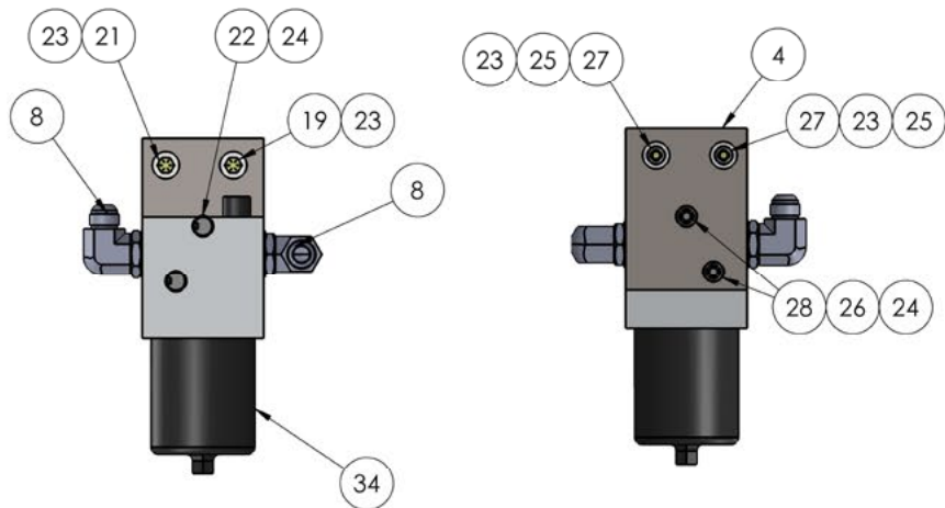
HIGH PRESSURE FILTER (FRONT & BACK)
