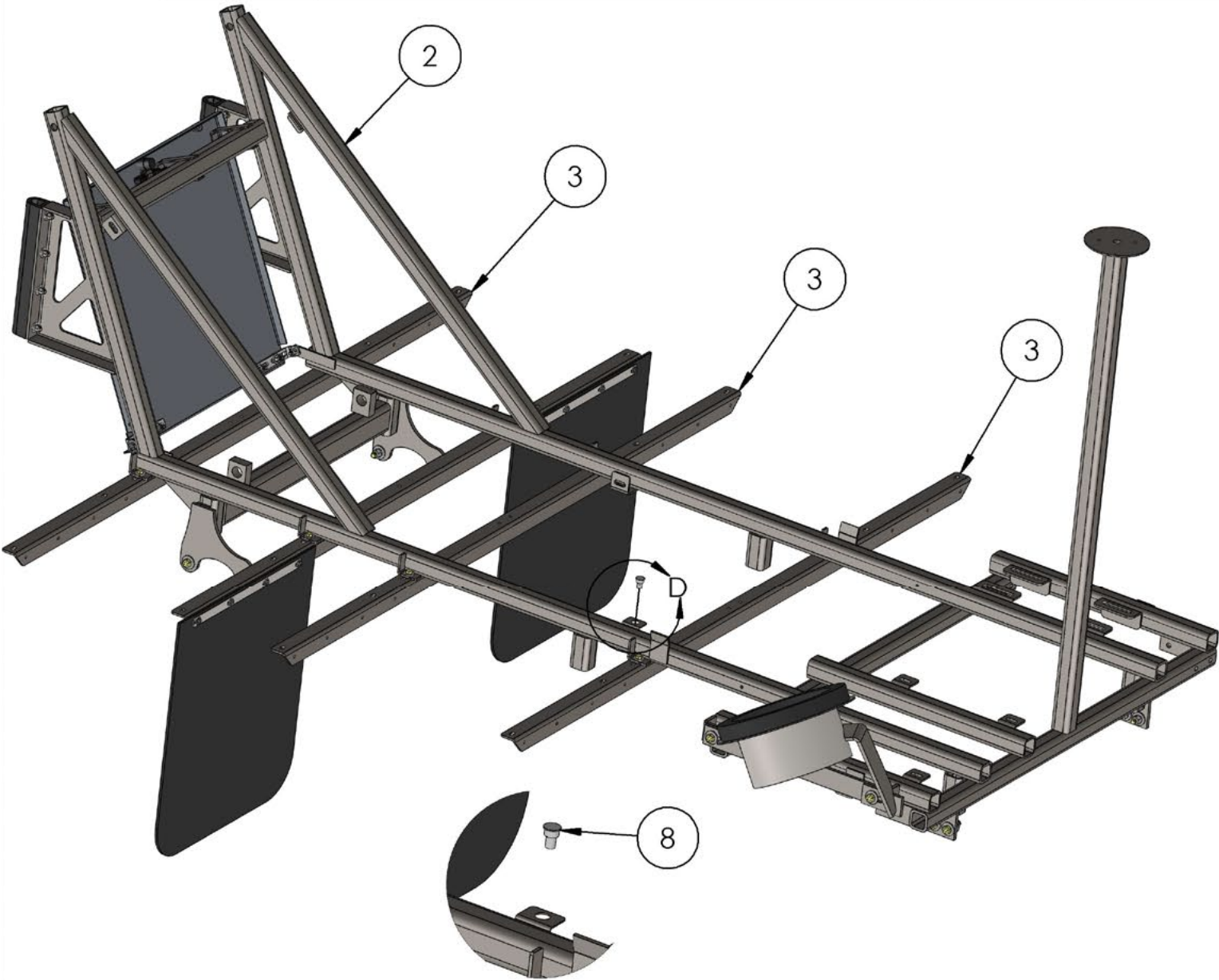
Front View Dump Frame - Diagram 1
