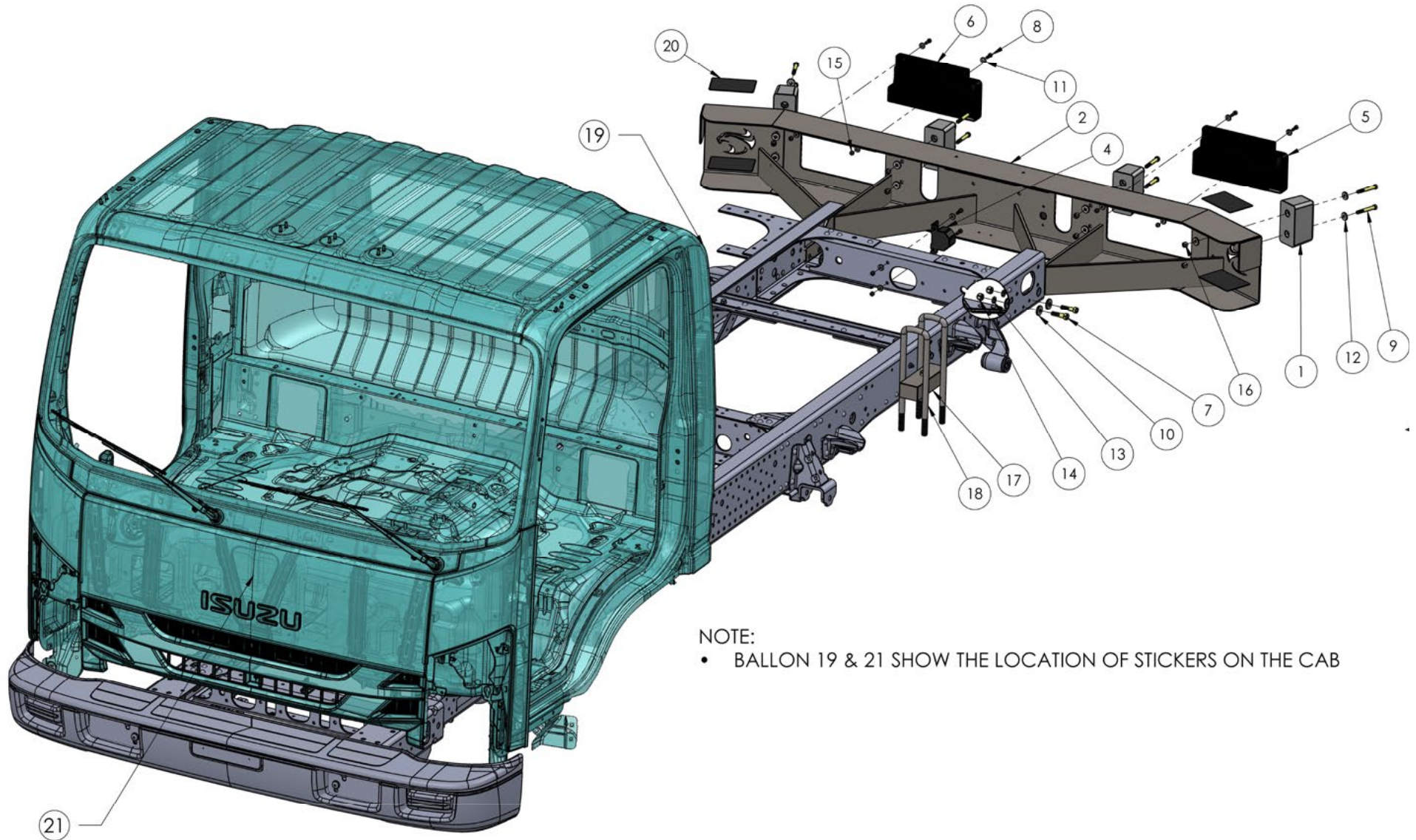
Side View - Rear Bumper Assembly - Diagram 1
