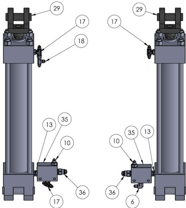
HOPPER LIFT CYLINDERS
