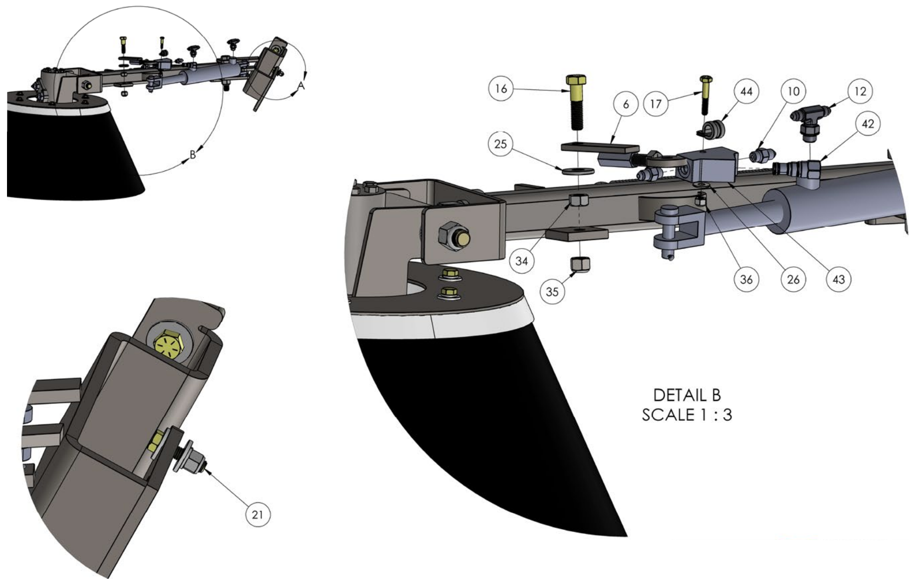
CB Arm - Cylinder Attachment - Diagram 3
